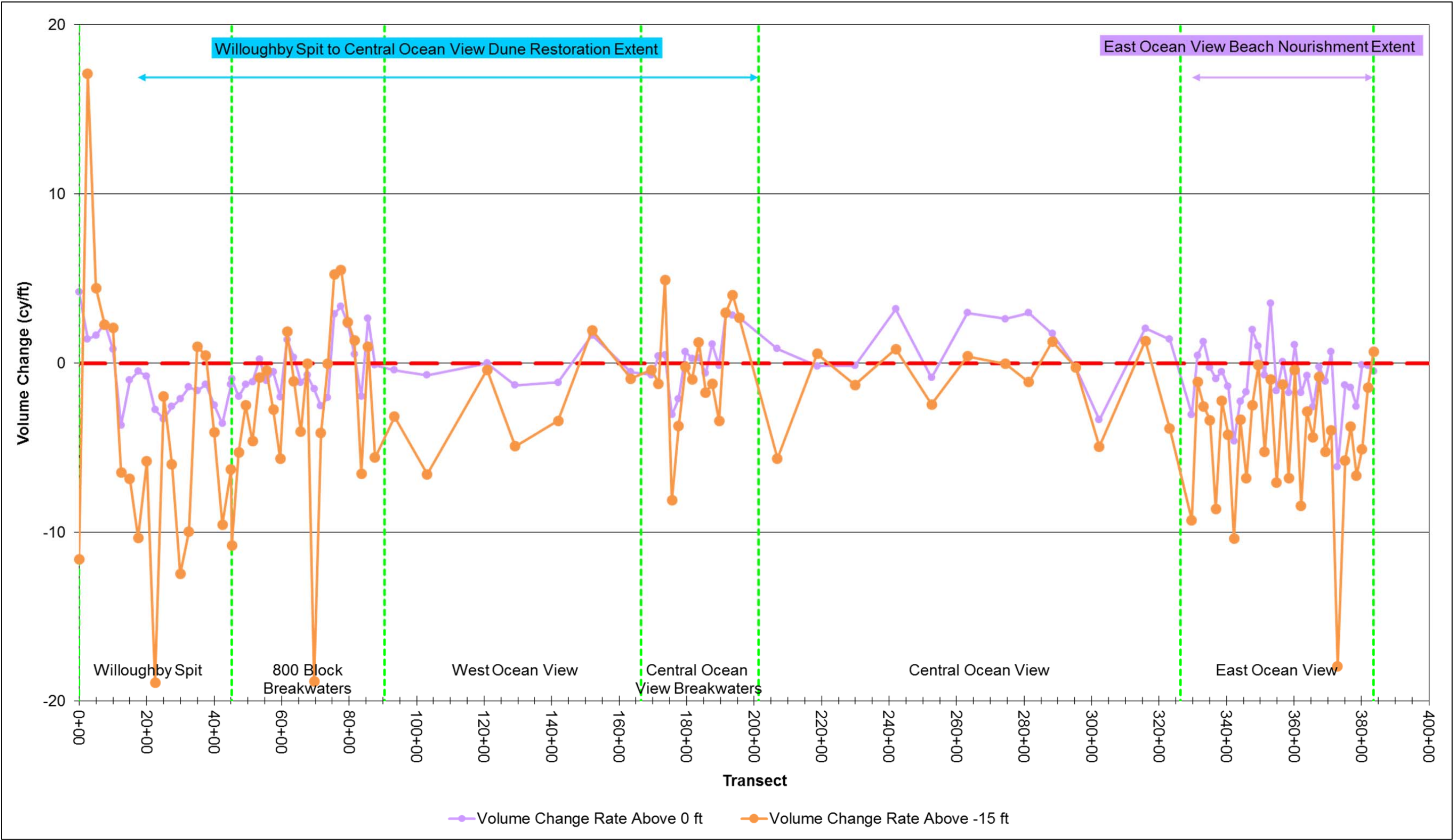
Figure 5-4: Volume Change Above 0 ft NAVD88 (cy/ft) and -15 ft NAVD88 for March 2012 to September 2012 (Note: Positive = Accretion, Negative = Erosion)
