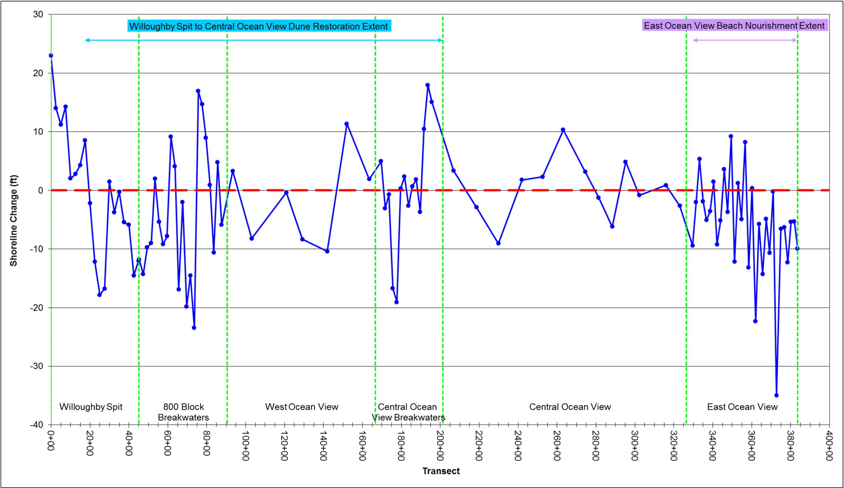
Figure 5-3: Shoreline Change (ft) at Mean High Water (+0.98 ft NAVD88) for March 2012 to September 2012 (Note: Positive = Accretion, Negative = Erosion)
