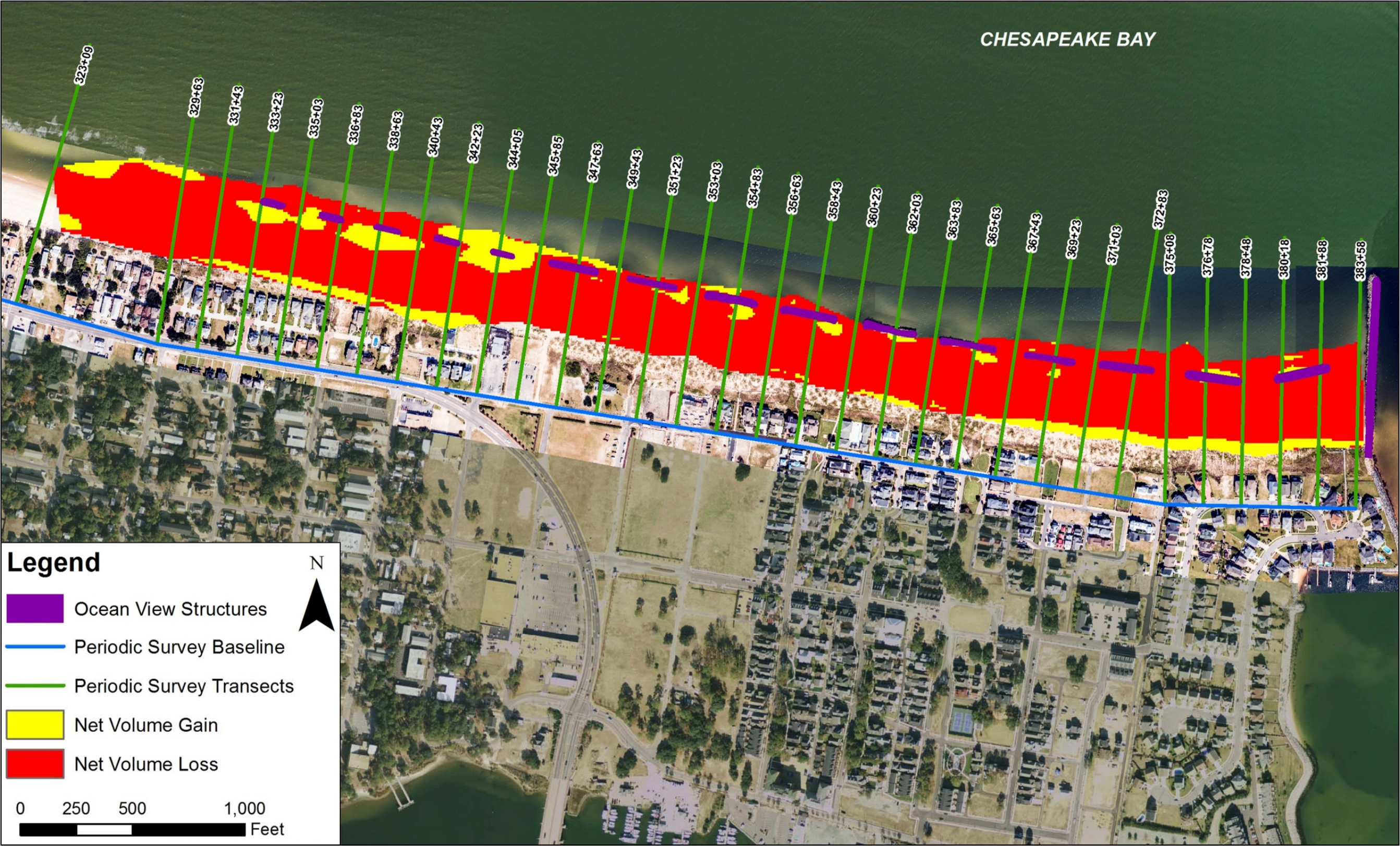
Figure 5-5: Net Volume Change Since the East Ocean View Nourishment Project (March 2009)
