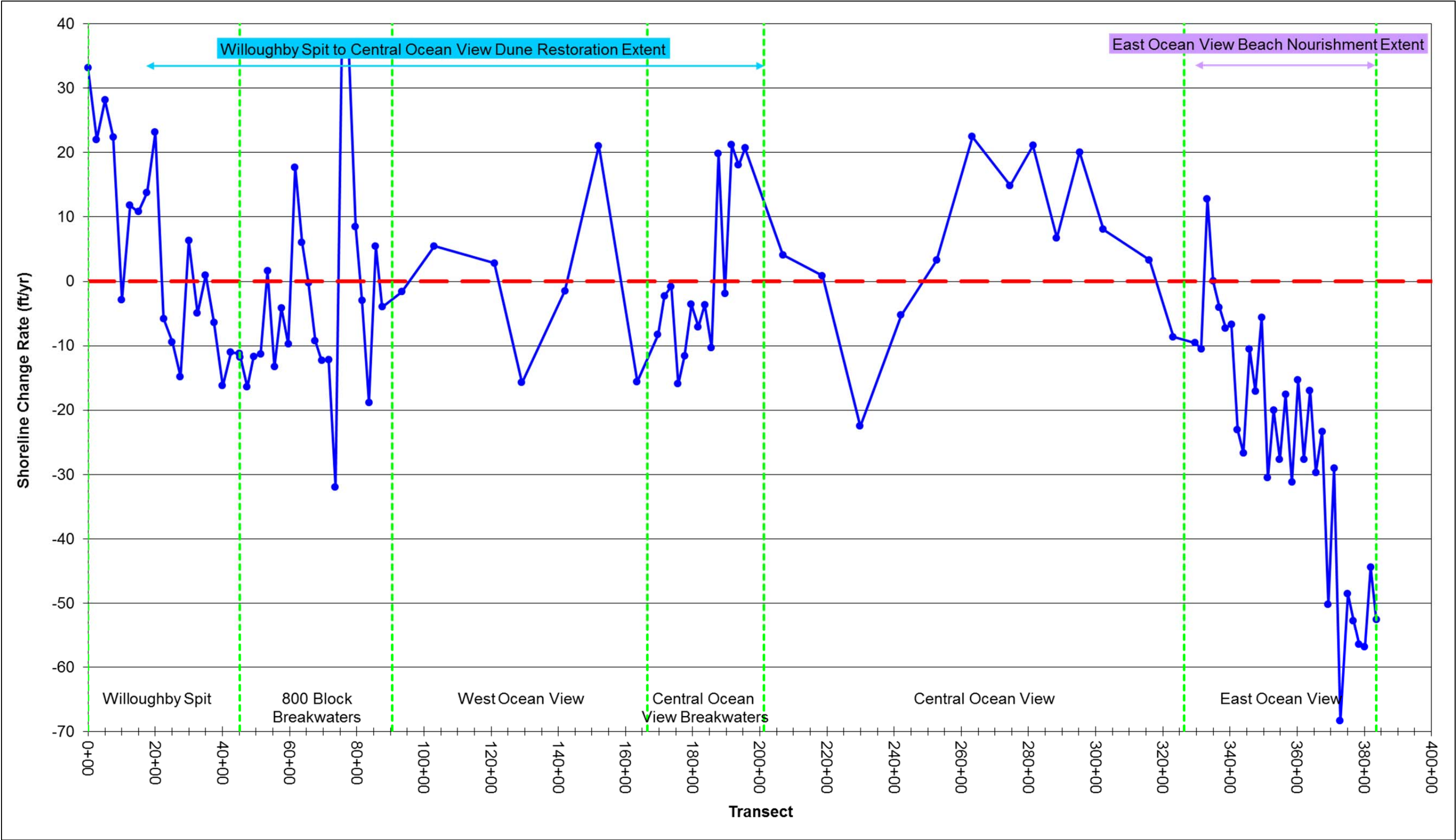
Figure 5-1: Shoreline Change Rate (ft/yr) at Mean High Water (+0.98 ft NAVD88) for October 2011 to September 2012 (Note: Positive = Accretion, Negative = Erosion)
