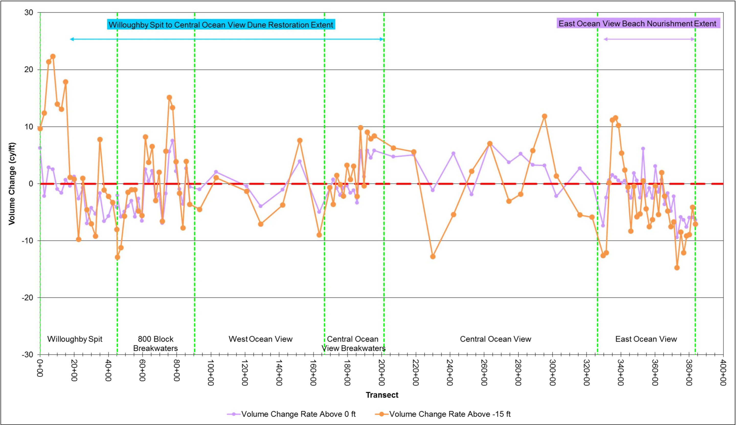
Figure 5-2: Volume Change Rate Above 0 ft NAVD88 (cy/ft) for October 2011 to September 2012 (Note: Positive = Accretion, Negative = Erosion)
